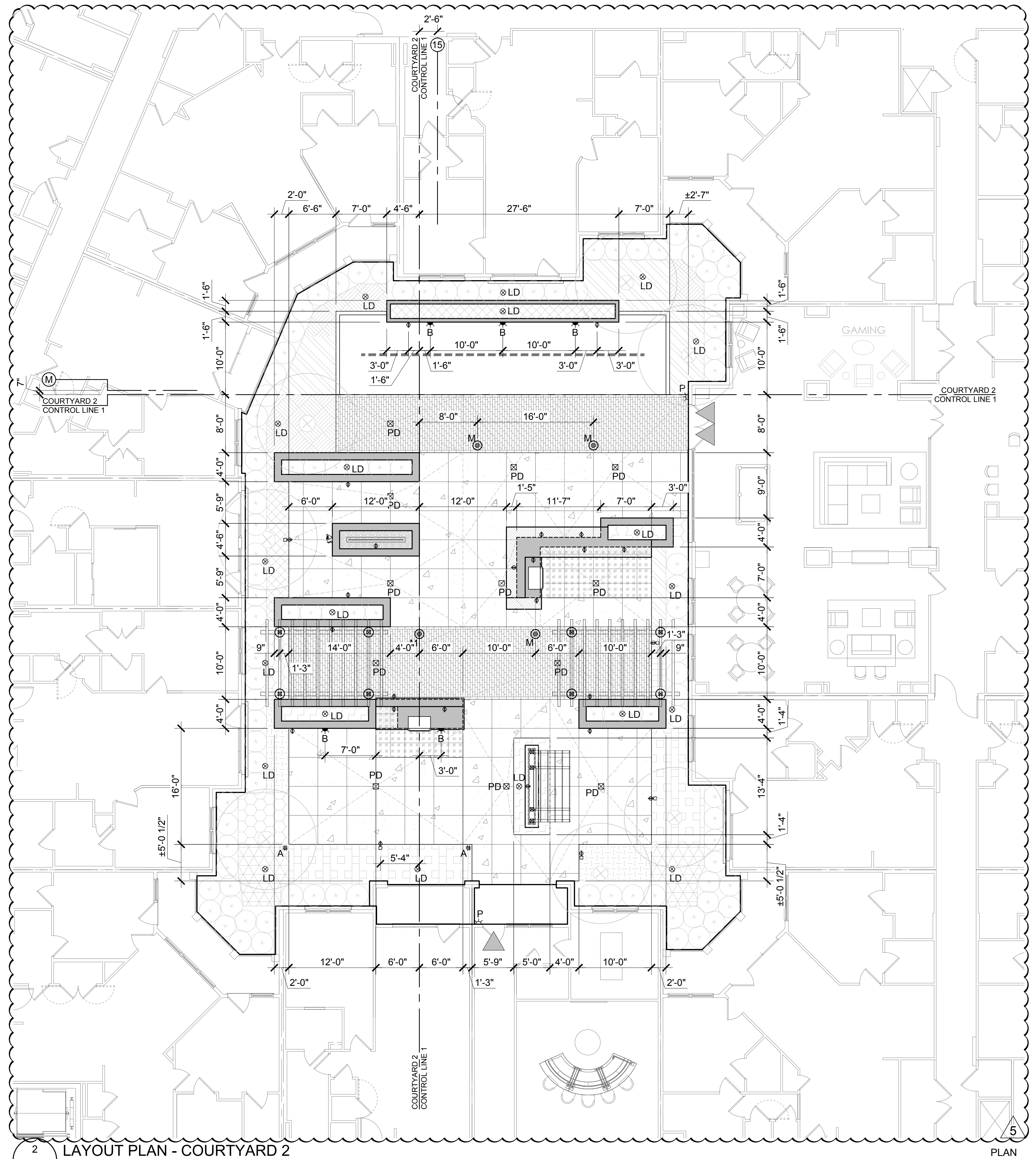
2 LAYOUT PLAN - COURTYARD 2 L1.08 Scale: 1/8" = 1'-0"
