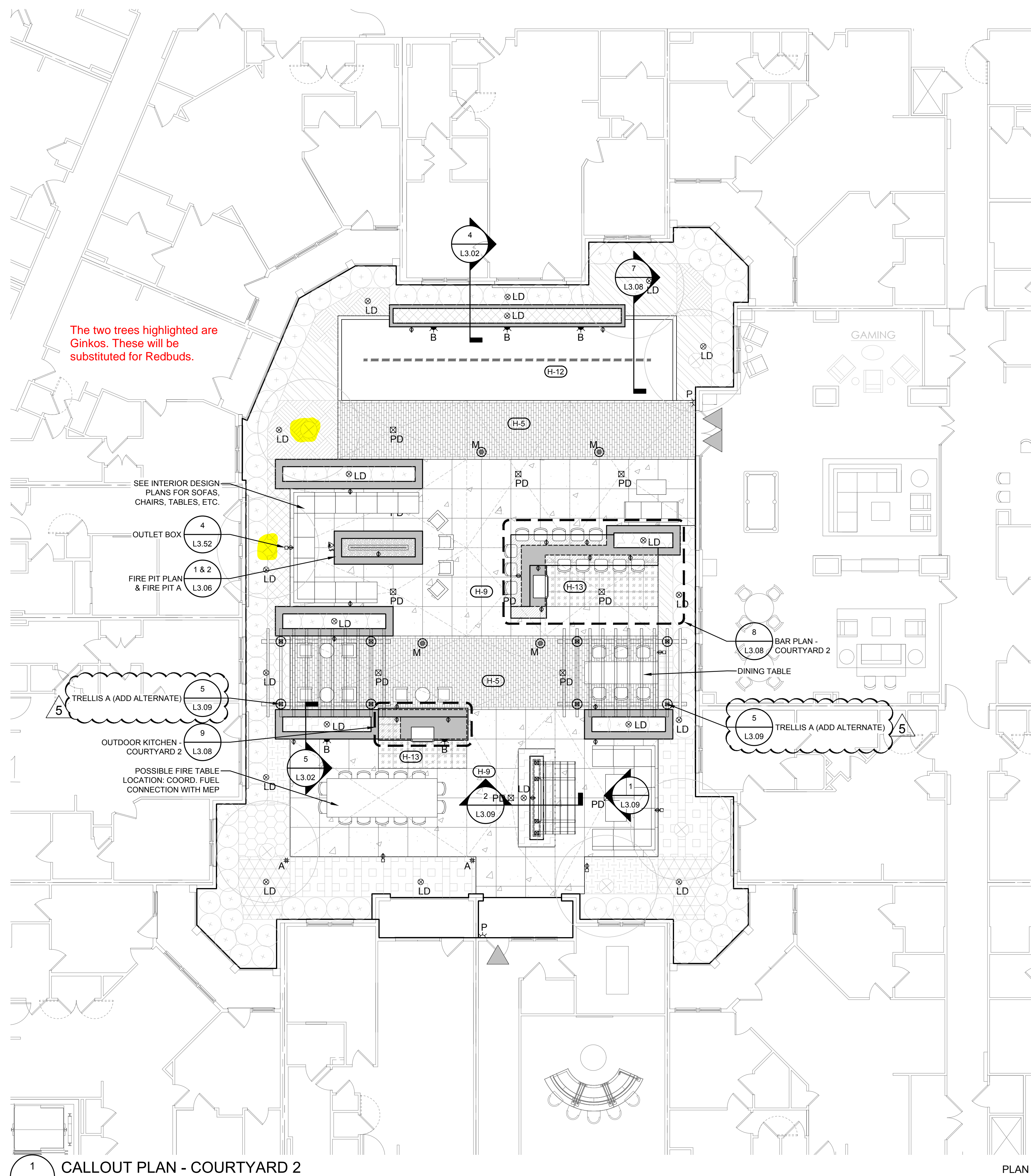
1 CALLOUT PLAN - COURTYARD 2 L1.08 Scale: 1/8" = 1'-0"
