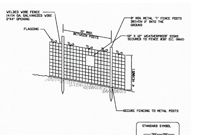
Tree Protection Fence Detail Not to scale
