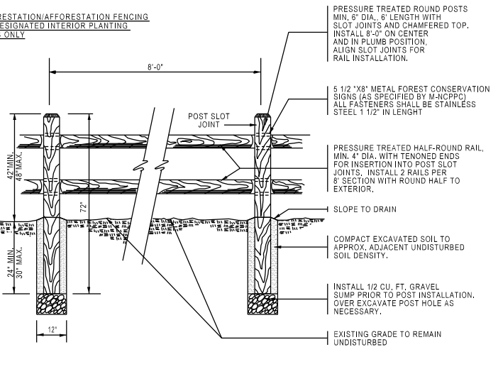
SPLIT RAIL FENCE DETAIL NOT TO SCALE
