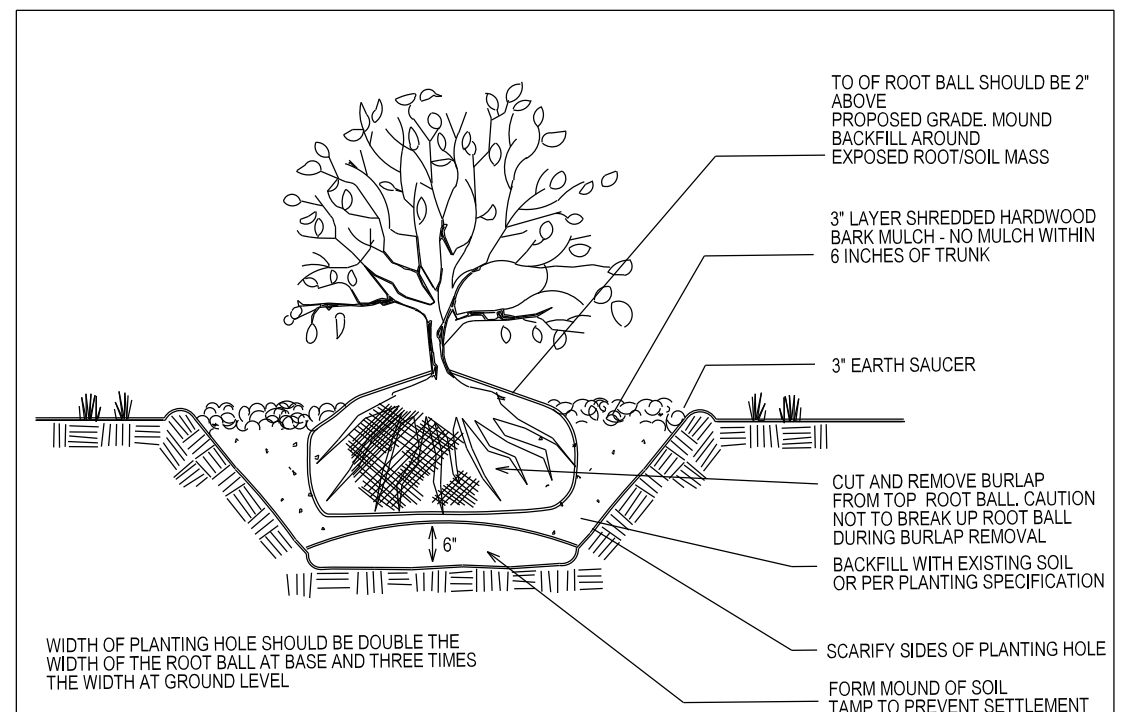
SHRUB PLANTING DETAIL BALLED AND BURLAPPED NTS
