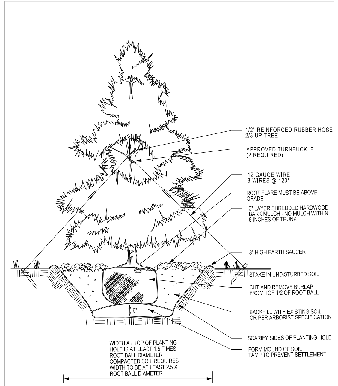
EVERGREEN PLANTING DETAIL BALLED AND BURLAPPED NTS
