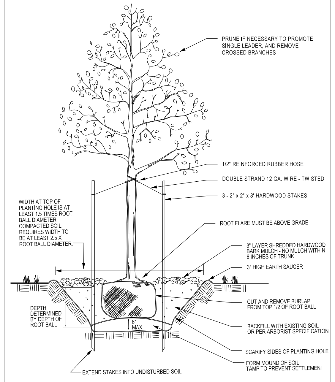
TREE PLANTING DETAIL BALLED AND BURLAPPED NTS
