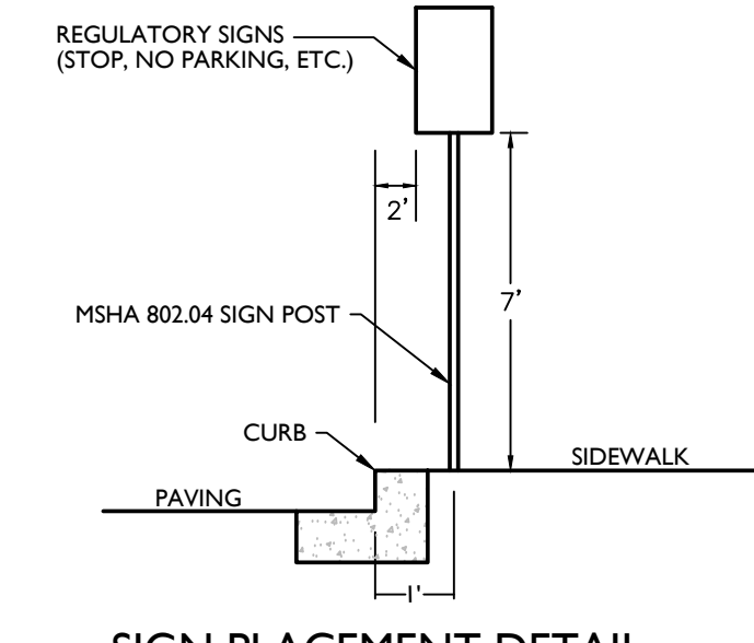
SIGN PLACEMENT DETAIL N.T.S.
