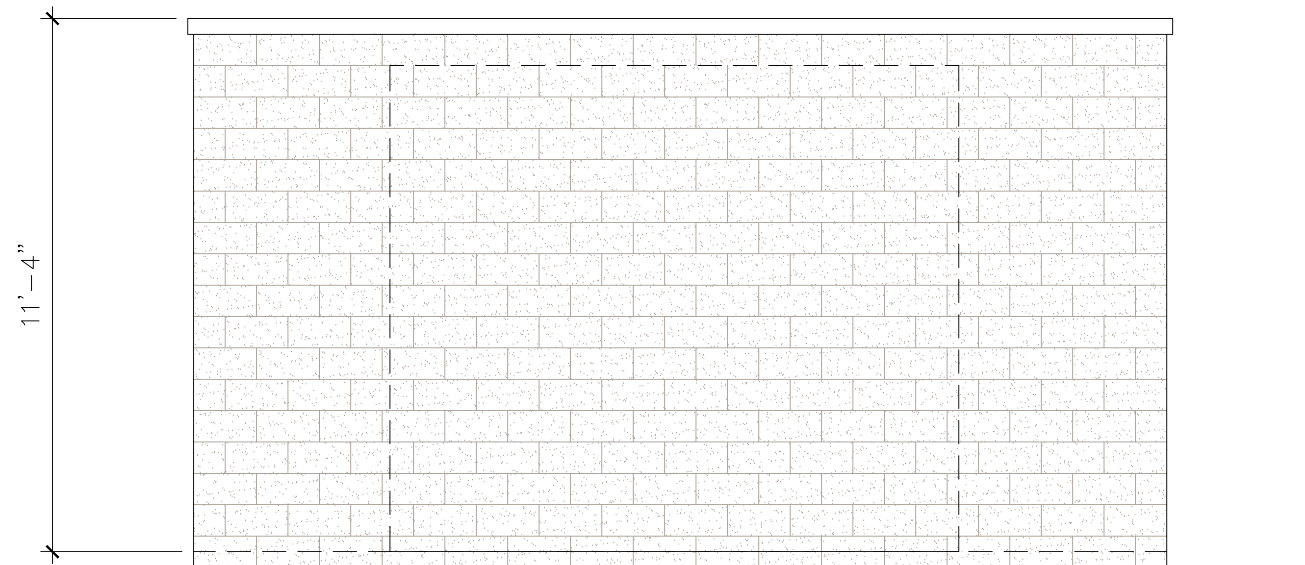
3 - Generator Enclosure - Side Elevation (Typ.) Scale: 1/2" = 1'-0"
