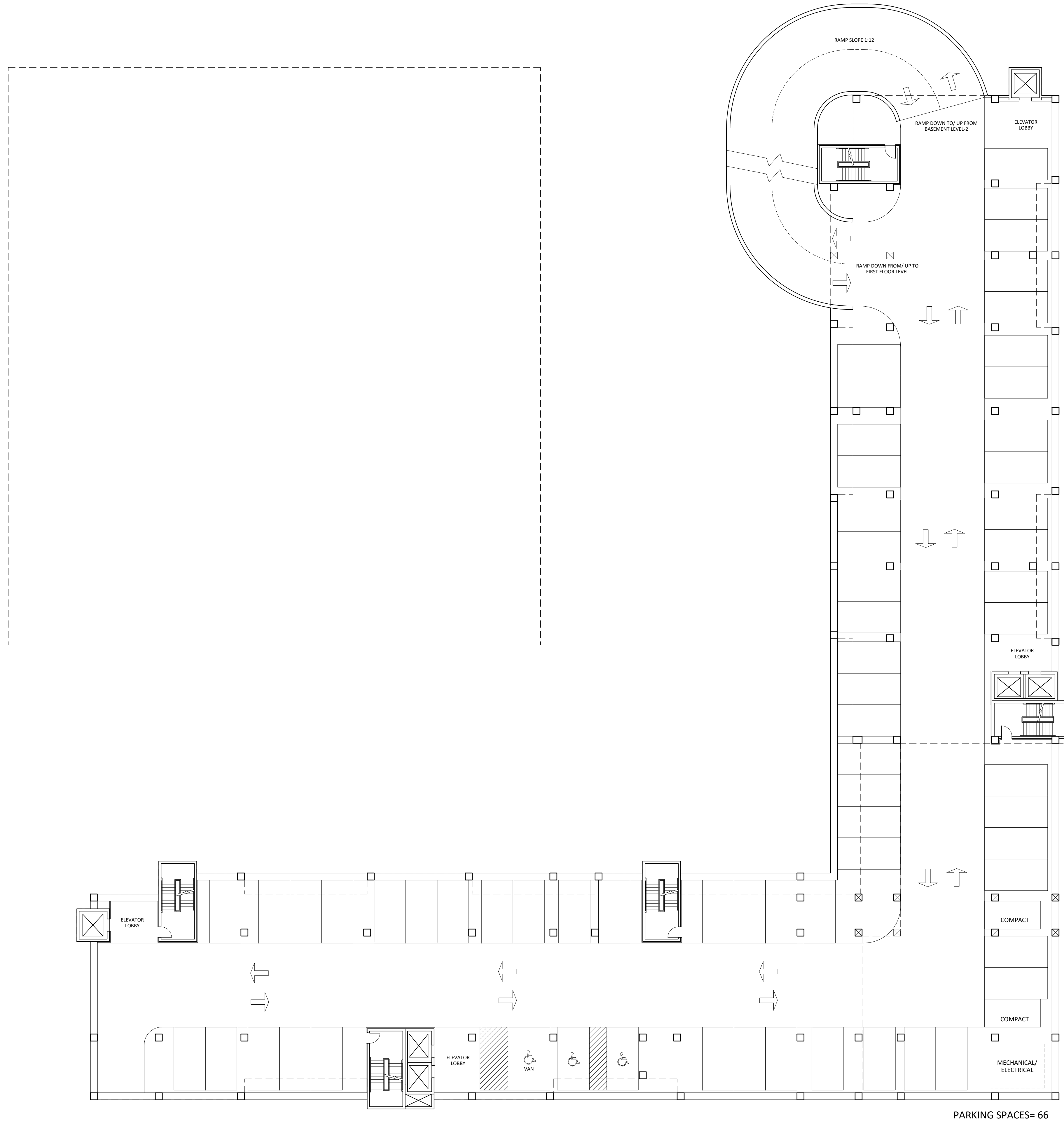
BASEMENT LEVEL-1 FLOOR PLAN
