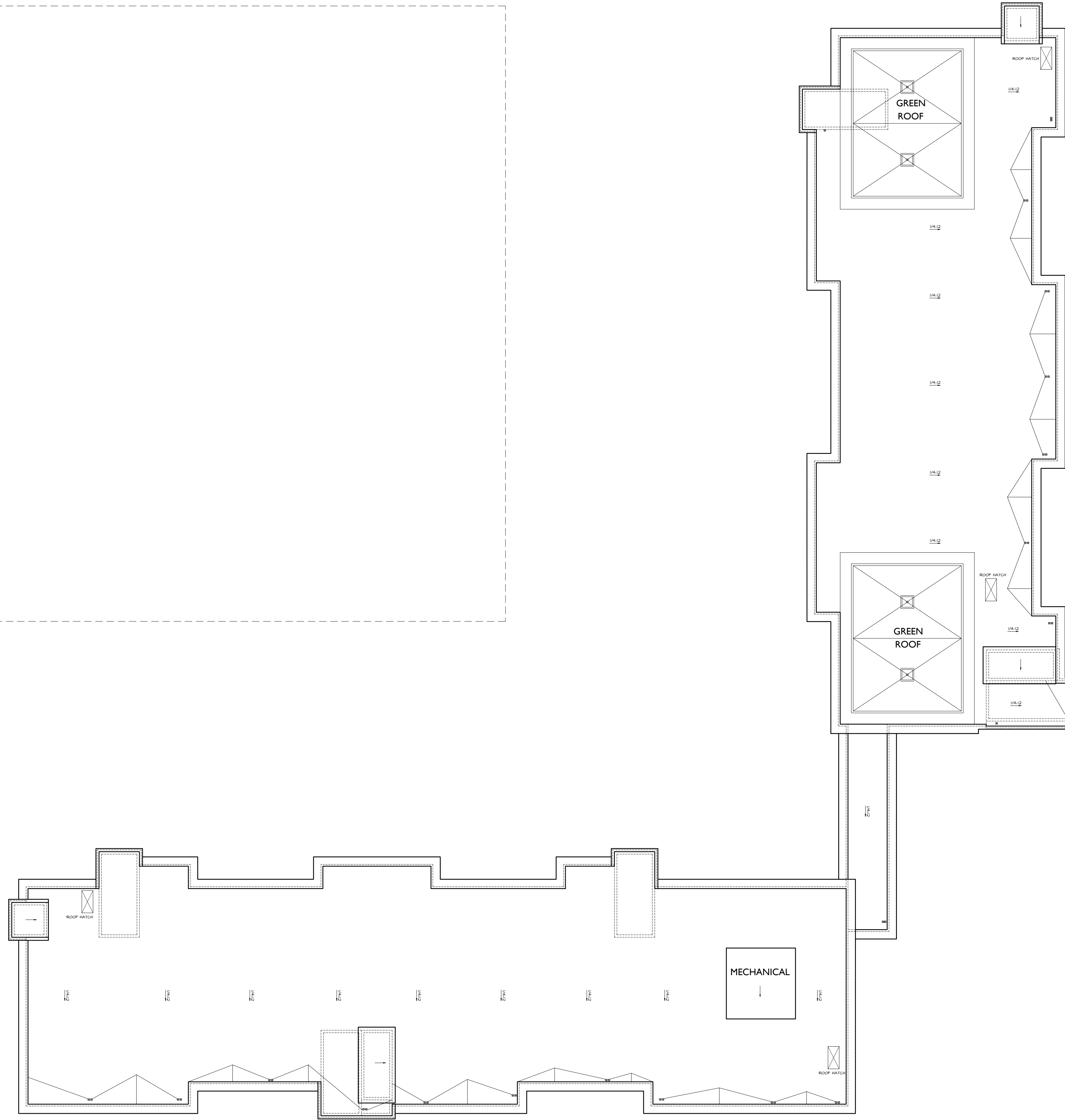
ROOF PLAN 1/8" = 1'-0"
