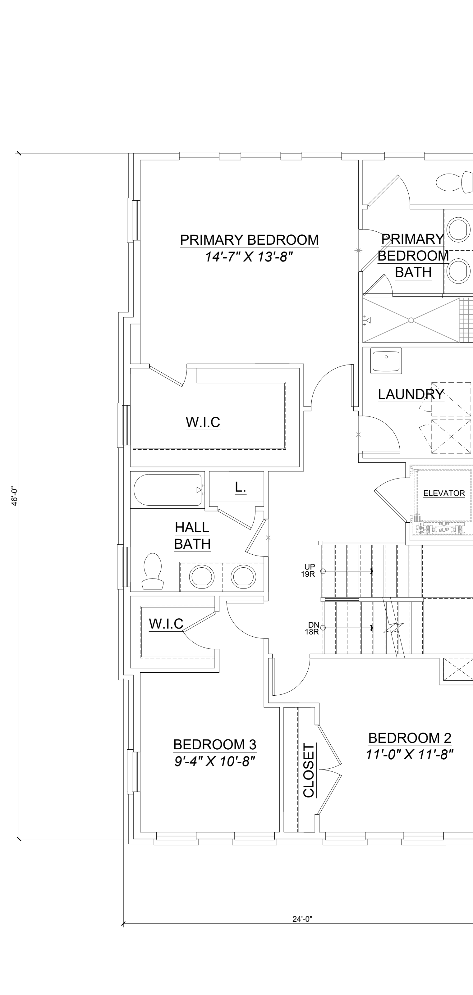
THIRD FLOOR PLAN (9' CLG) (1089 SQ. FT..)
