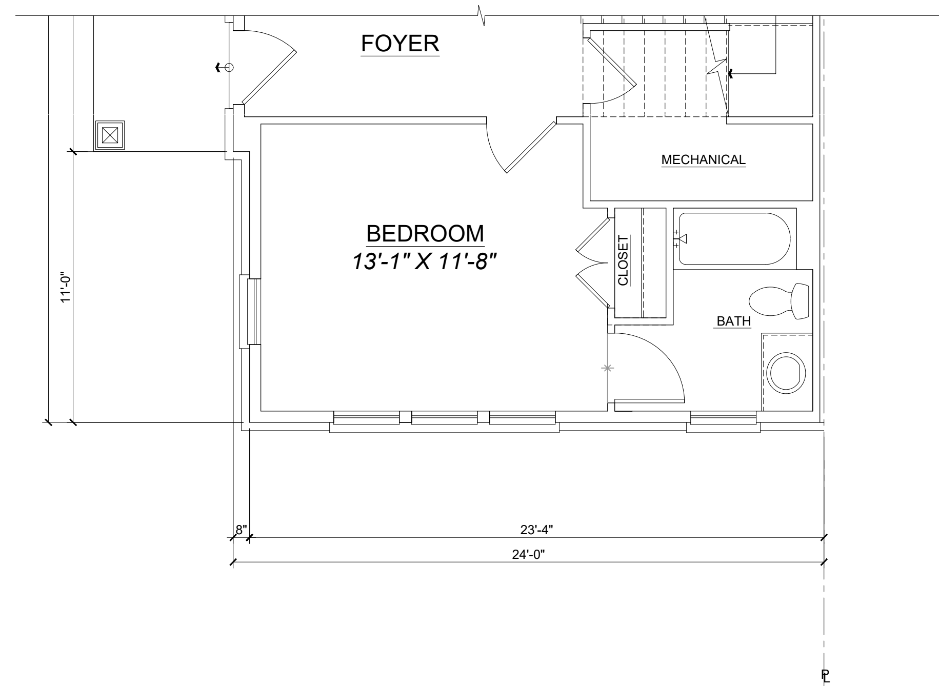
PARTIAL FIRST FLOOR PLAN OPT. BEDROOM
