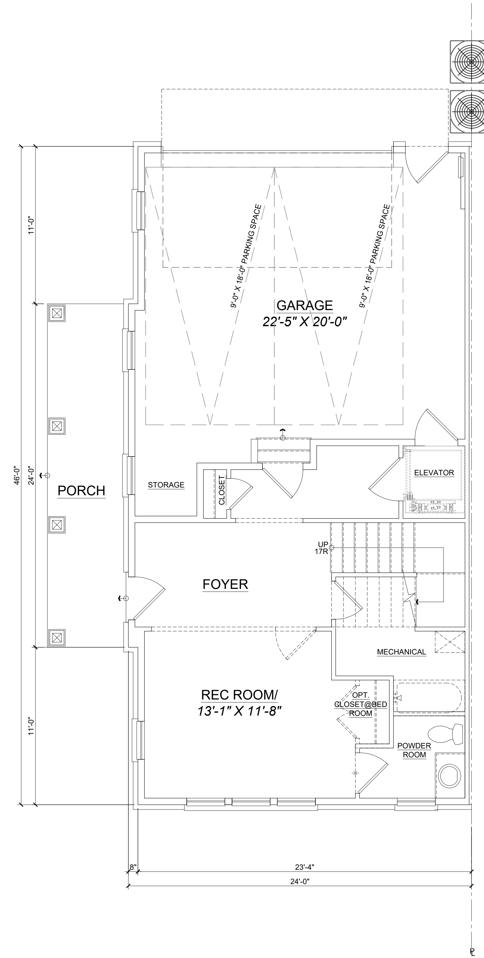
FIRST FLOOR PLAN (9' CLG)- 574 SQ. FT. (2- CAR GARAGE )-516 SQ. FT.
