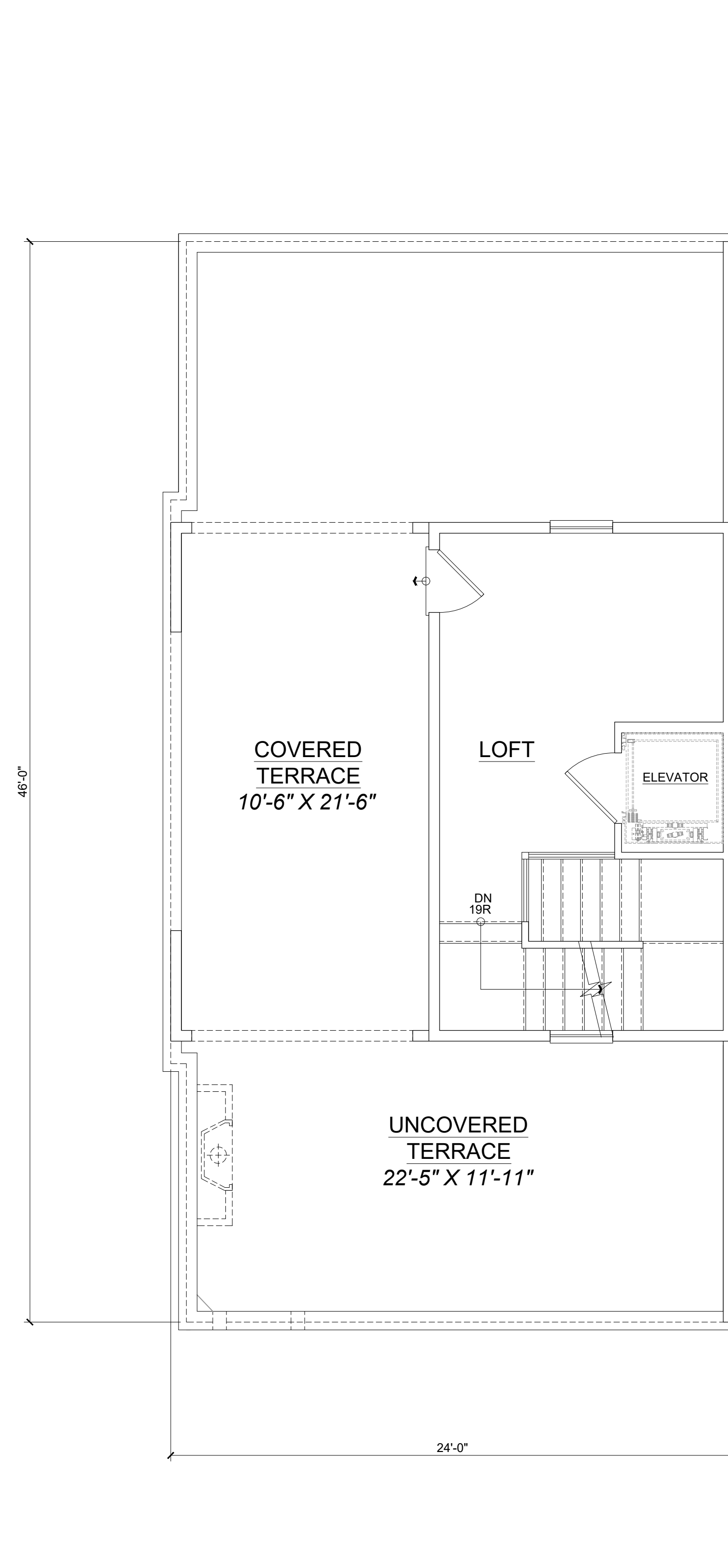
FOURTH FLOOR PLAN (8' CLG) (209 SQ. FT.) (OPTIONAL TERRACE #1 243 SQ. FT.) (OPTIONAL TERRACE #2 279 SQ. FT.)
