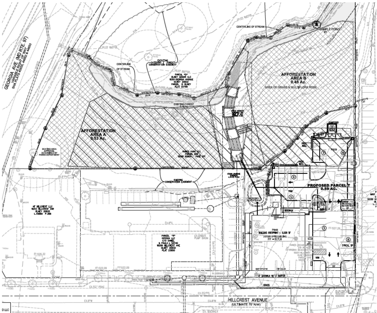
Figure 3 – Tree Save Plan (Excerpt)
