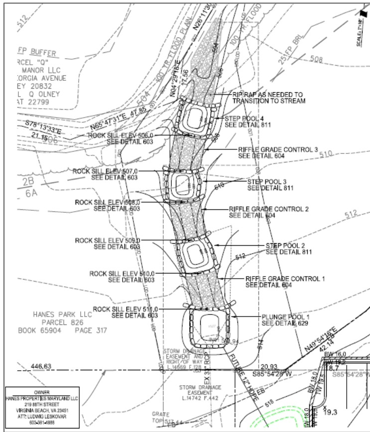
Figure 4 – Stormwater Outfall Detail (Excerpt)
