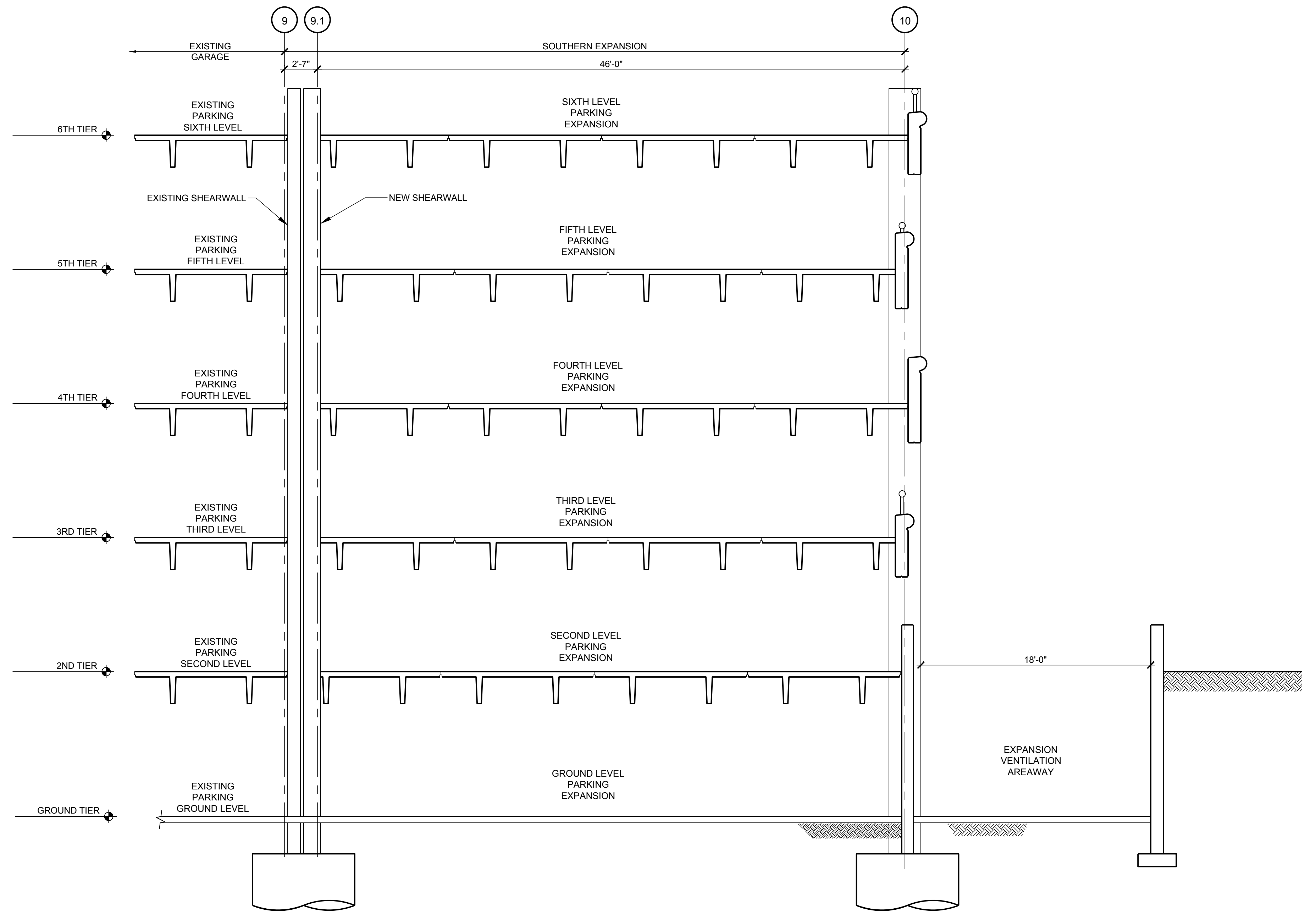
2 SECTION LOOKING EAST (SOUTHERN EXPANSION)
